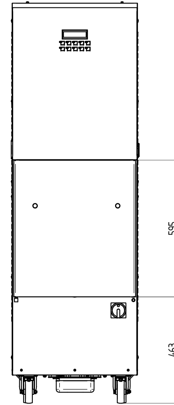
REAR VIEW
