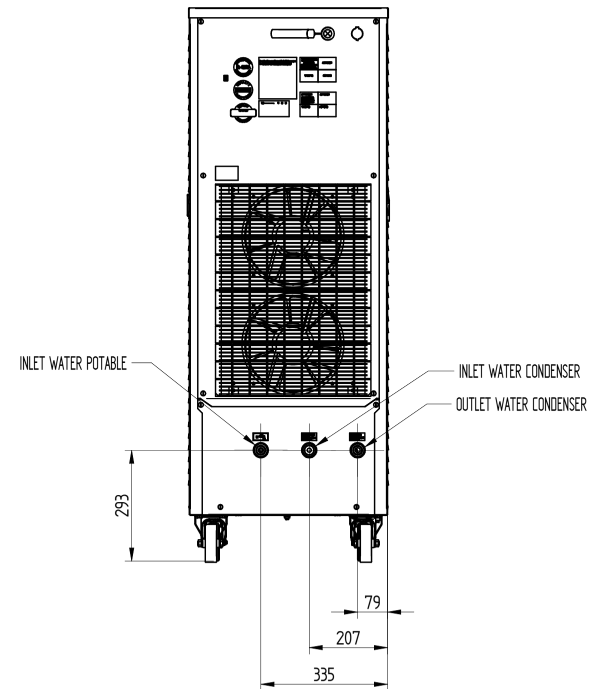
REAR VIEW
