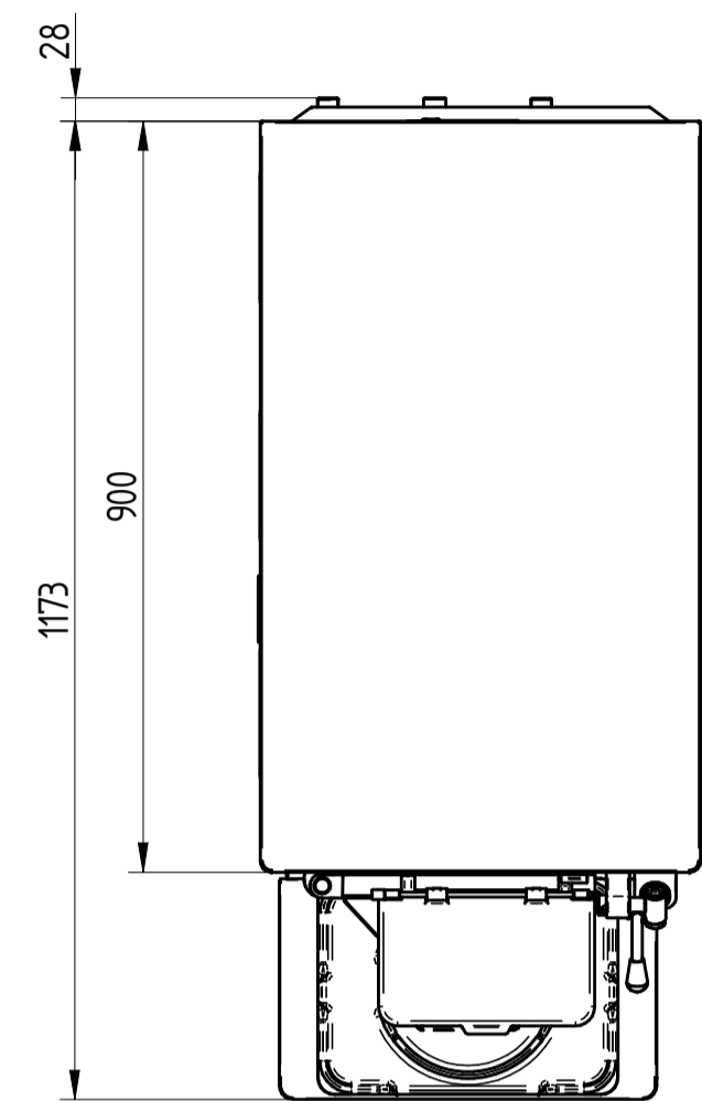
UPPER VIEW
