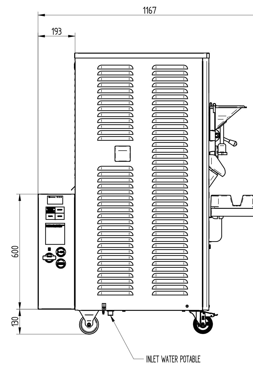
LEFT SIDE VIEW AIR VERSION
