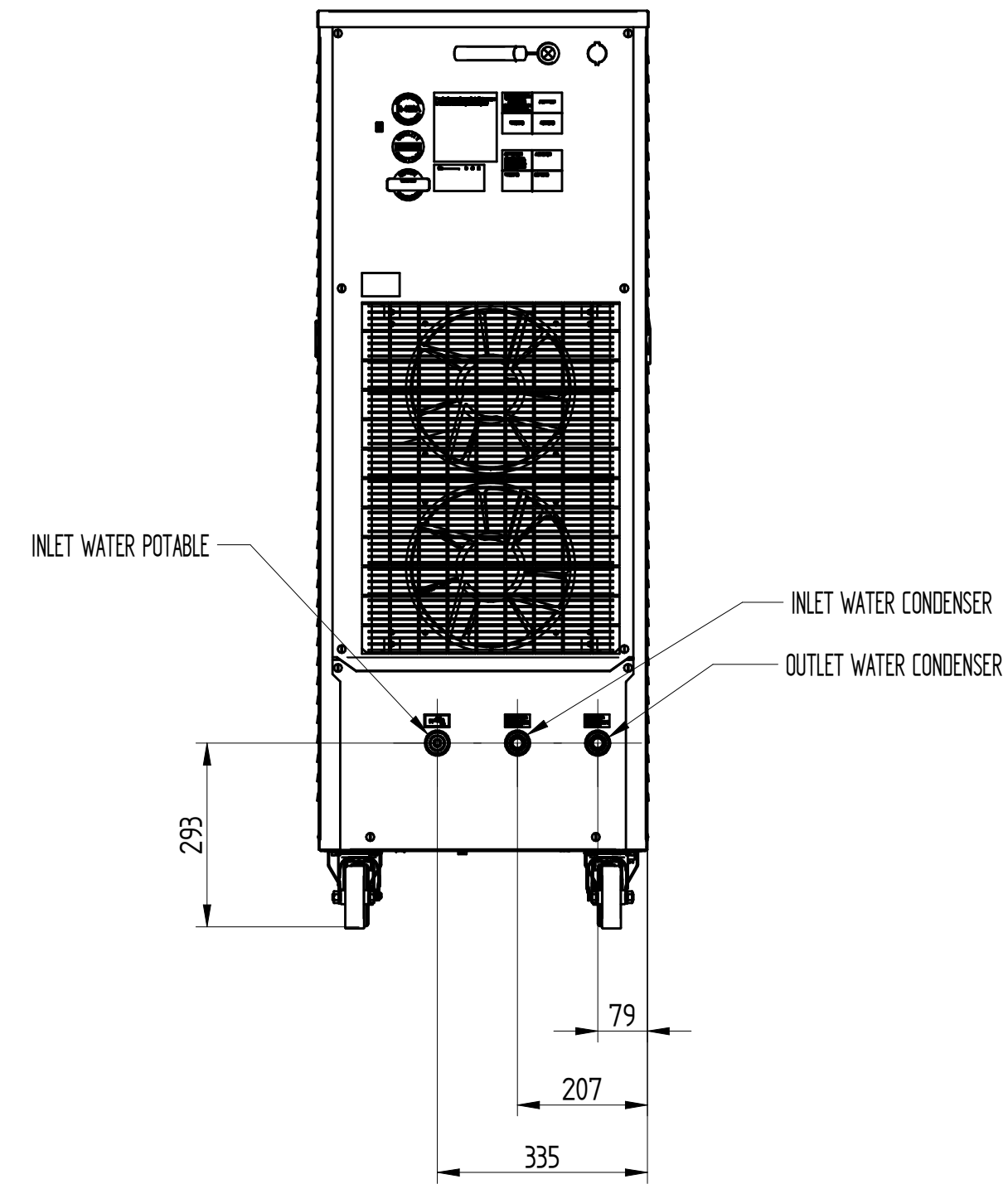
REAR VIEW
