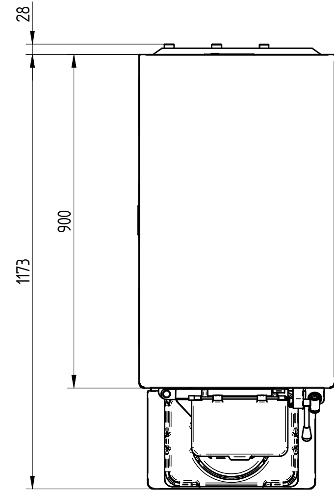
UPPER VIEW
