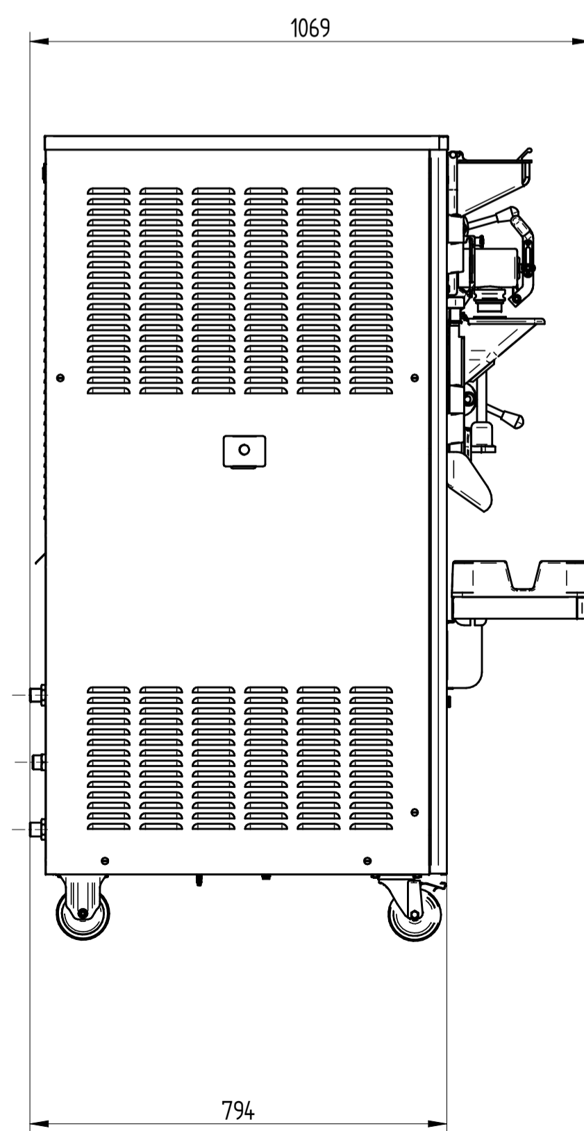
LEFT SIDE VIEW WATER VERSION
