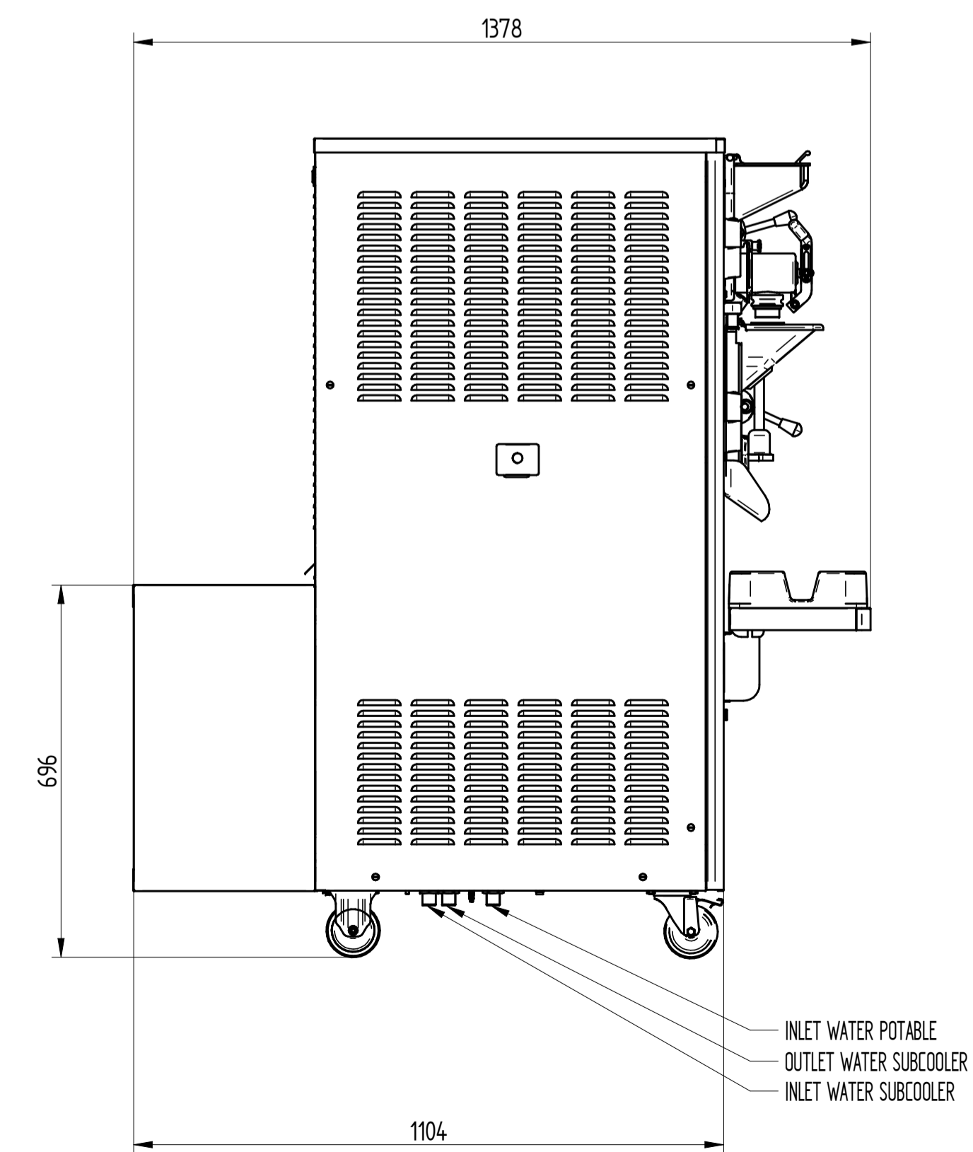
LEFT SIDE VIEW AIR VERSION
